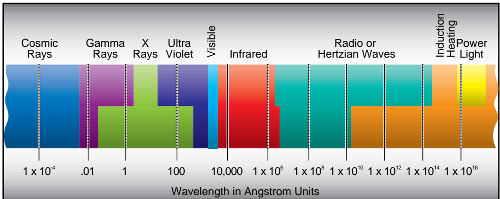
Figure 1 - Electromagnetic spectrum
