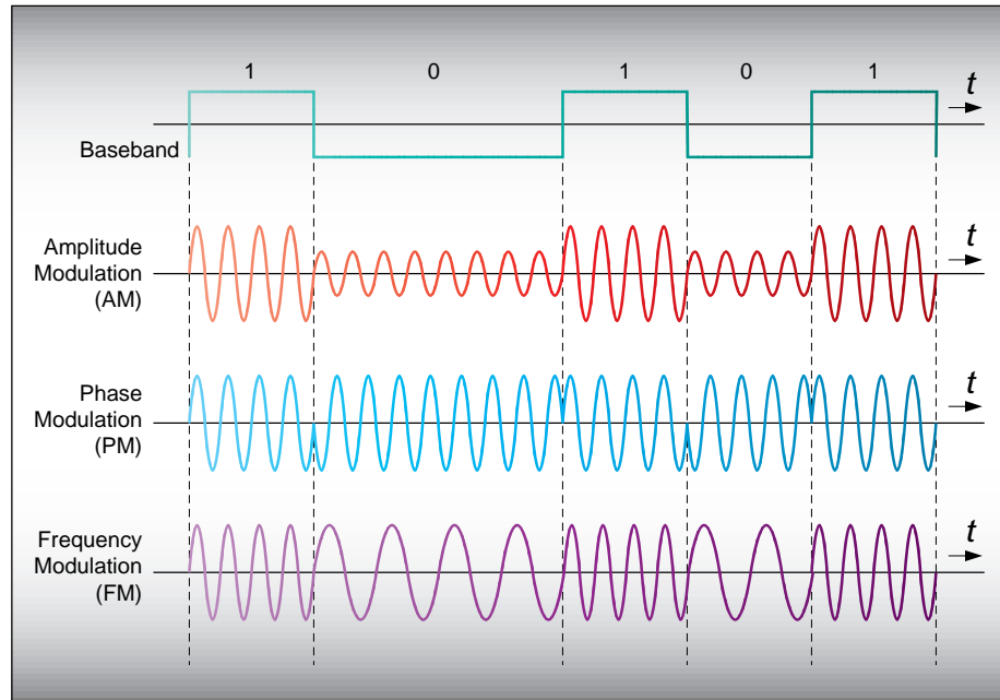
Figure 5 – Modulation waveforms
