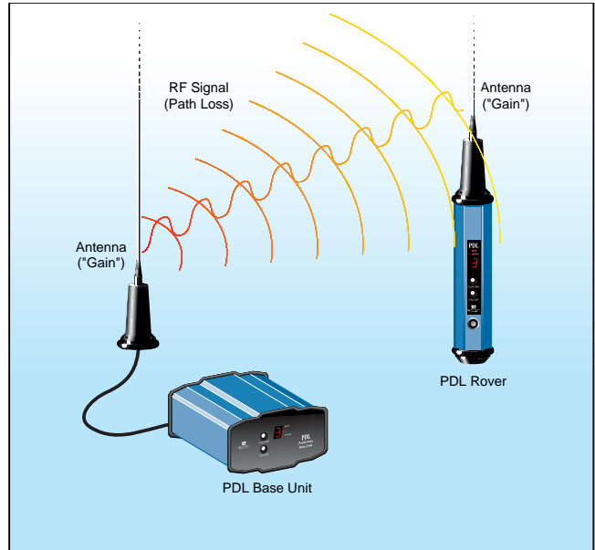
Figure 8 – Radio data link
