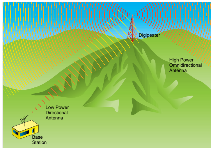
Figure 12 – Digipeater application
