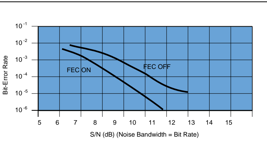
Figure 10 – Theoretical gain with FEC
