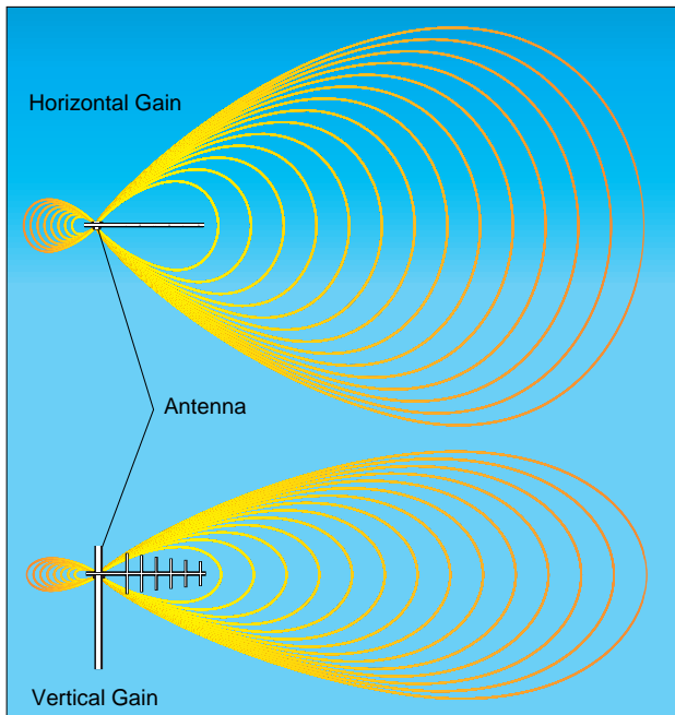
Figure 7 – Directional antenna gain pattern
