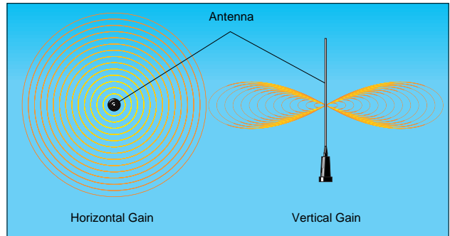
Figure 6 – Omni-directional antenna gain pattern
